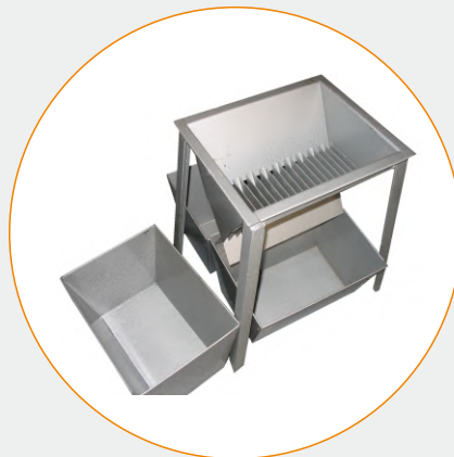
Sample Splitter
